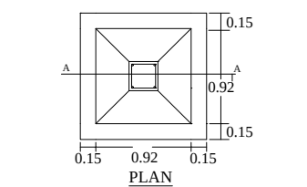
FOUNDATION DETAILS
