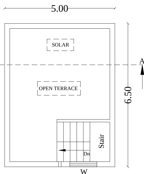
TERRACE FLOOR
