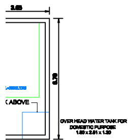
OVER HEAD WATER TANK FOR DOMESTIC PURPOSE 1.80 x 2.81 x 1.20
