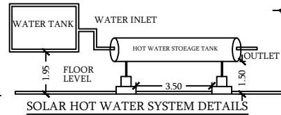
SOLAR HOT WATER SYSTEM DETAILS
