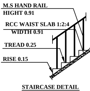
STAIRCASE DETAIL
