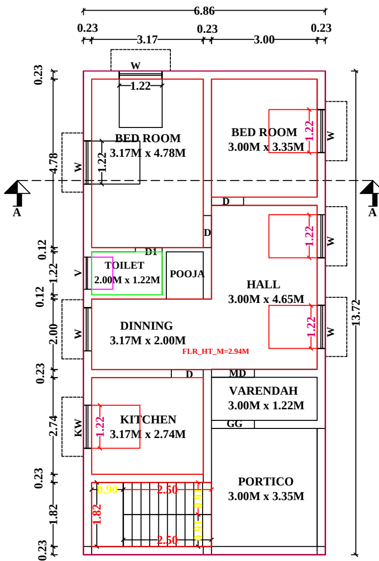
FLOOR-0
