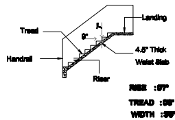
STAIRCASE DETAIL
