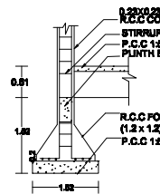
COLUMN DETAILS Size of column = 0.23m x 0.23m Not to scale
