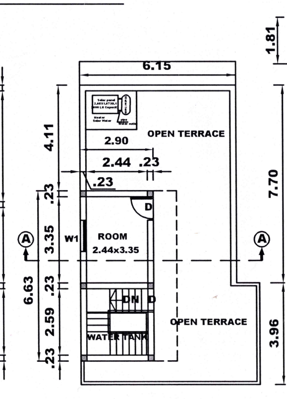
FIRST & TERRACE FLOOR PLAN
