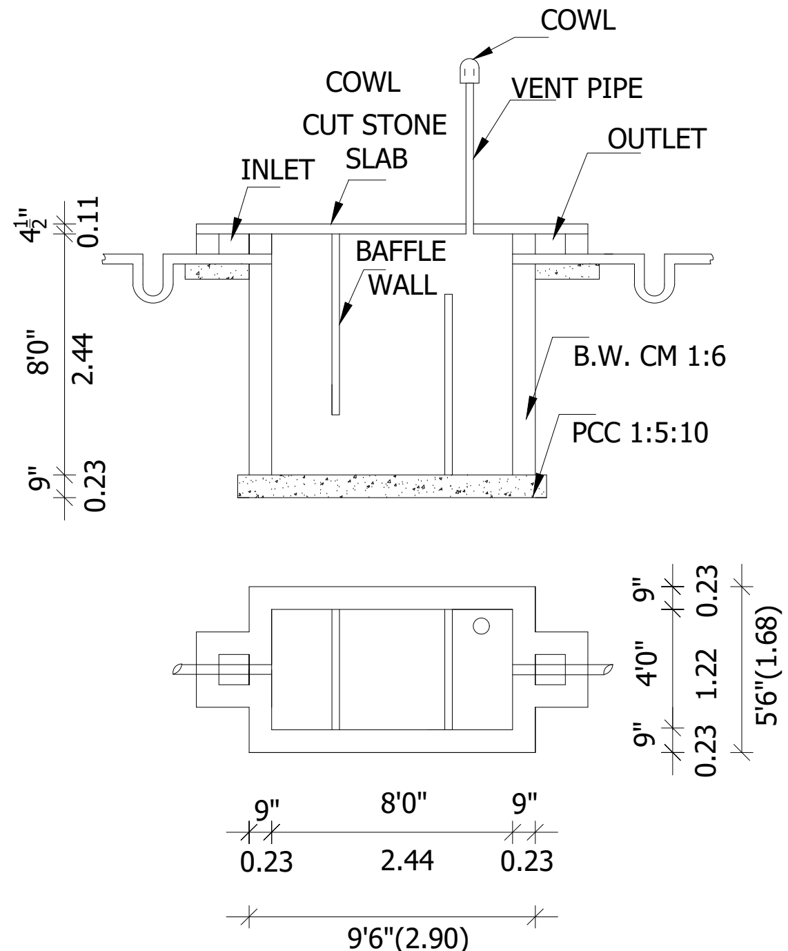
WASTE WATER RECYCLE UNIT
