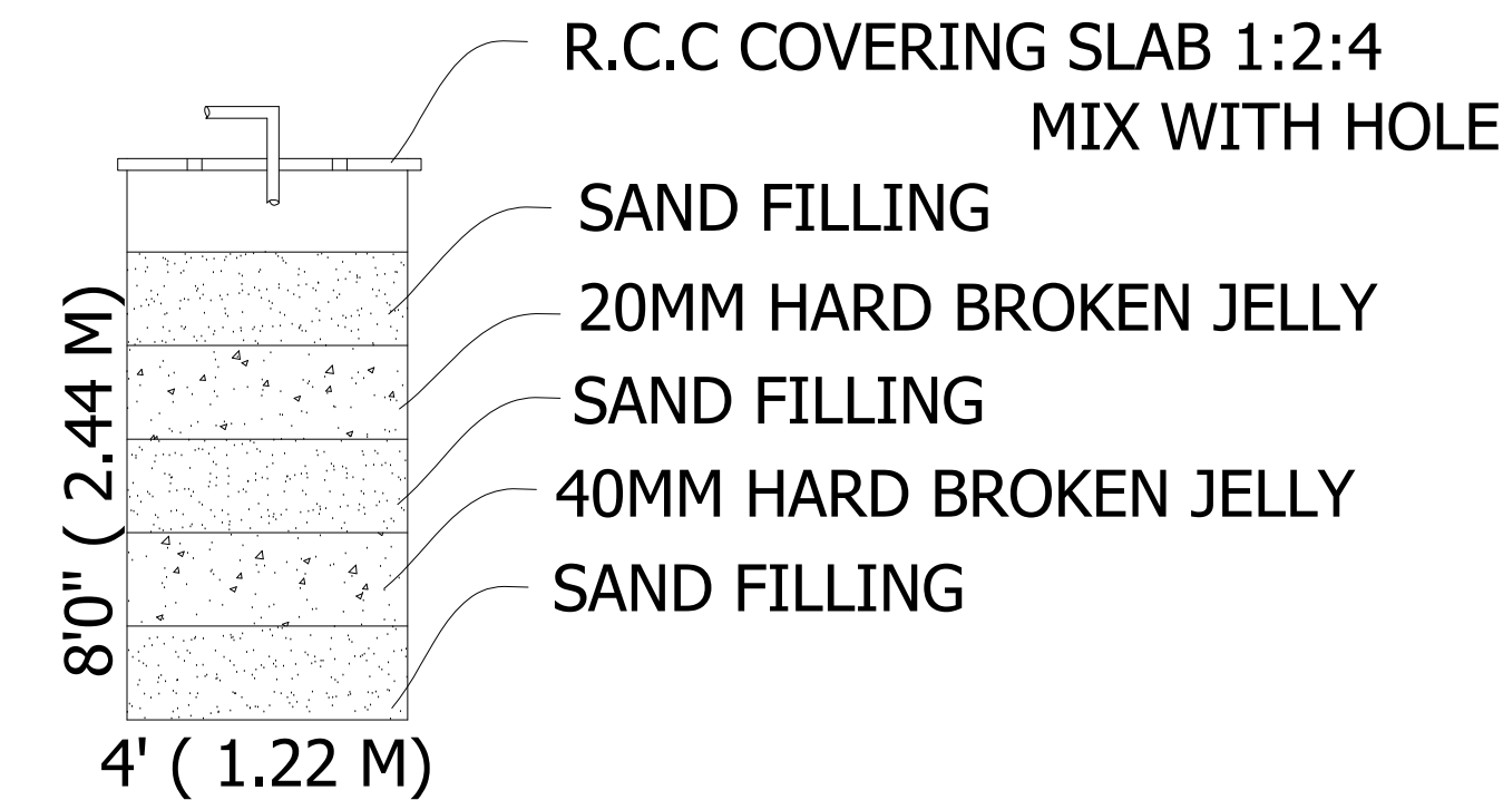
RAIN WATER HARVEST UNIT
