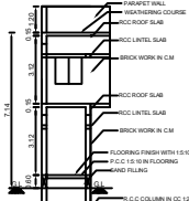
SECTION ON "AA"
