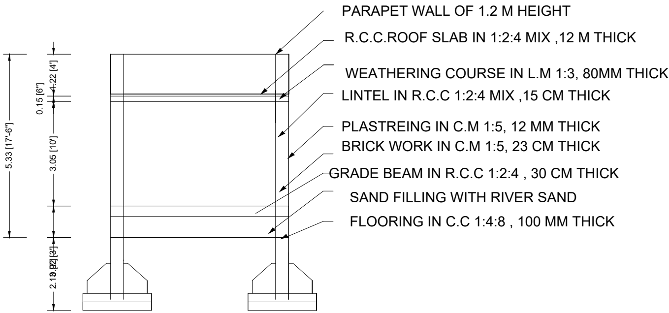
FOUNDATION DETAIL DESIGNED AS PER LOCAL SOIL CONDITION
