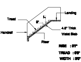
STAIRCASE DETAIL
