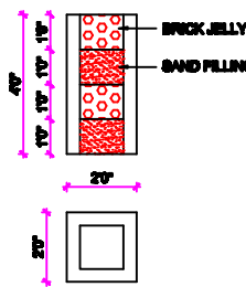
PERCOLATION TEST
