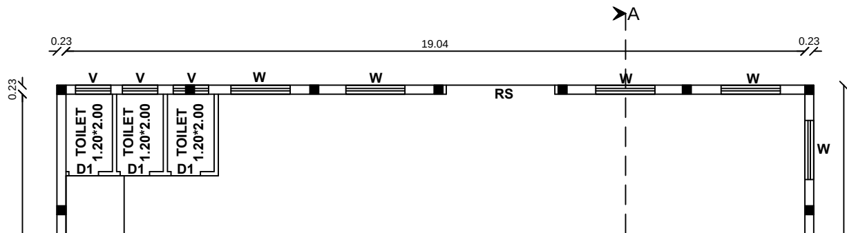
GODOWN 19.04*8.99
