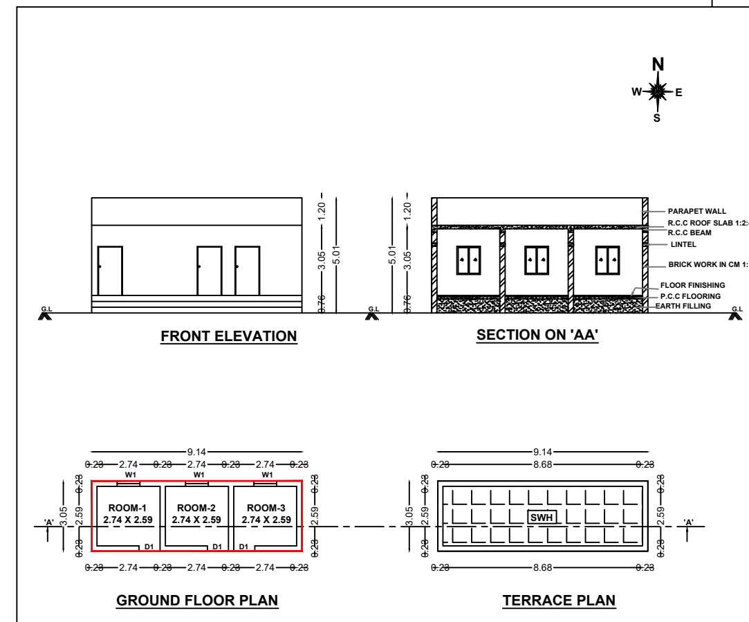
BLOCK -1 (LABOUR ROOM)
