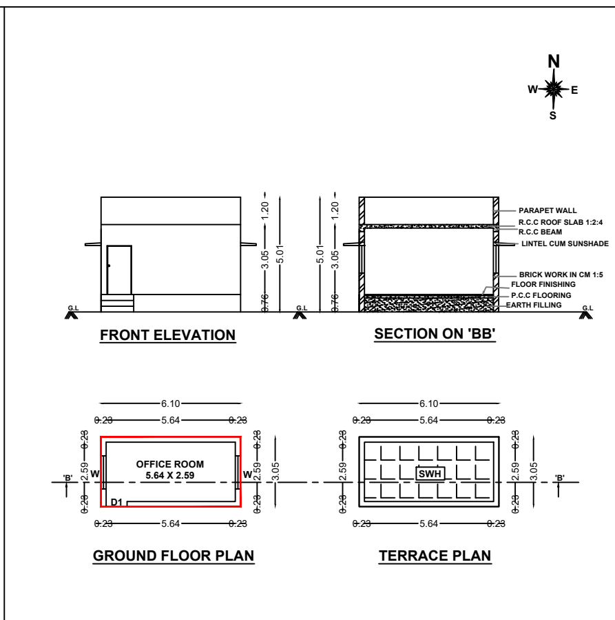
BLOCK -2 (OFFICE ROOM)
