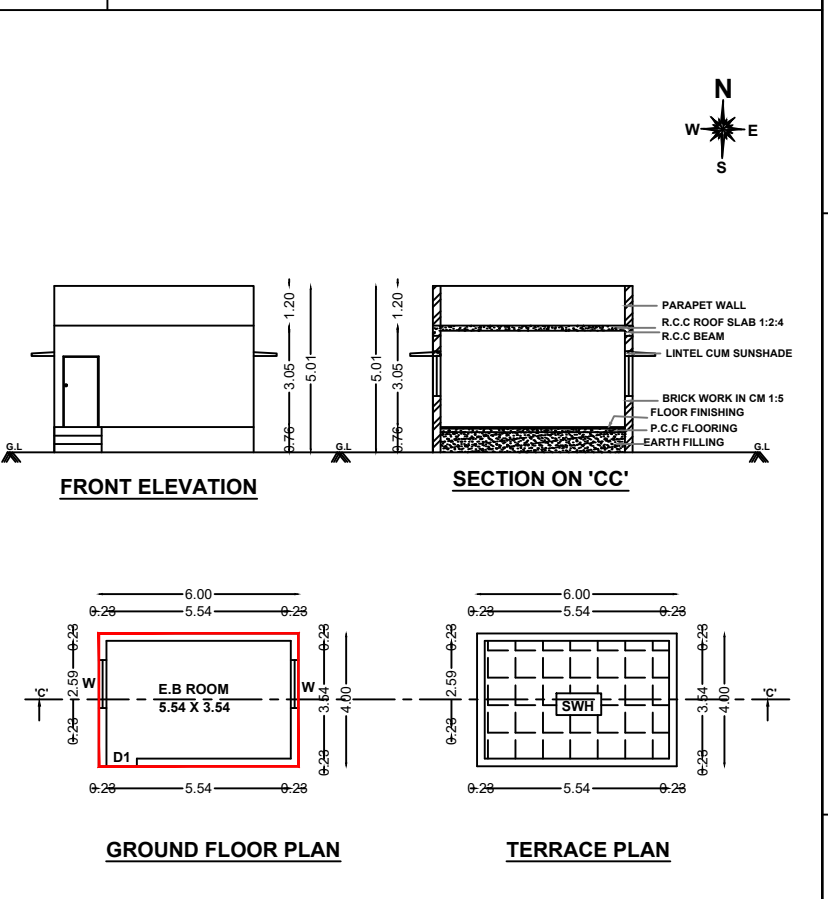
BLOCK -3 (EB ROOM)
