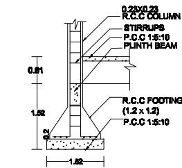
COLUMN DETAILS Size of column = 0.23m x 0.23m Not to scale
