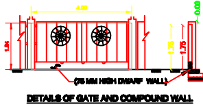
DETAILS OF GATE AND COMPOUND WALL
