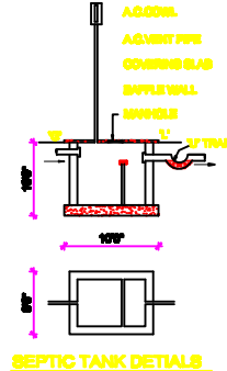
SEPTIC TANK DETAILS
