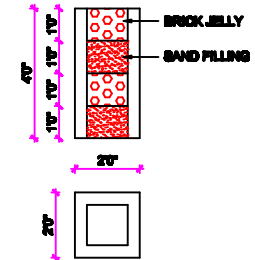
PERCUSSION PIT
