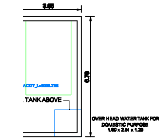
OVER HEAD WATER TANK FOR DOMESTIC PURPOSE
