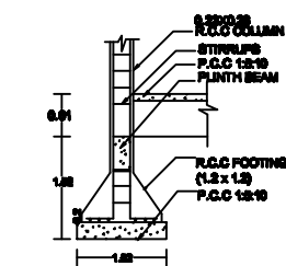
COLUMN DETAIL 8 Size of column = 0.23m x 0.23m Not to scale
