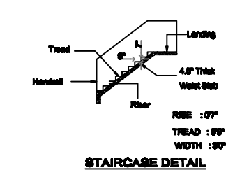
STAIRCASE DETAIL
