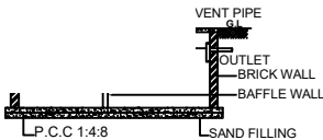
SECTION 'Y-Y'
