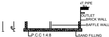
SECTION 'Y-Y'
