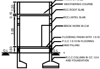
SECTION ON "AA"
