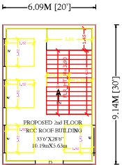
PROPOSED SECOND FLOOR PLAN
