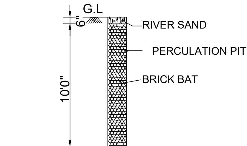
PERCOLATION PIT
