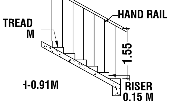
AIRCASE DETAILS
