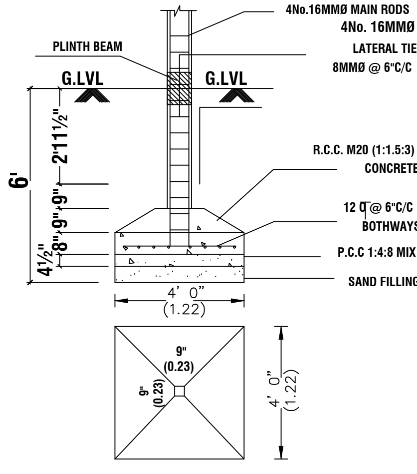
FOUNDATION DETAIL
