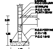
COLUMN DETAILS Size of column = 0.25m x 0.25m Not to scale
