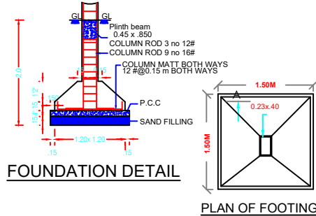
PLAN OF FOOTING
