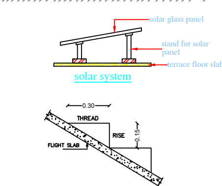
STAIRCASE DETAILS
