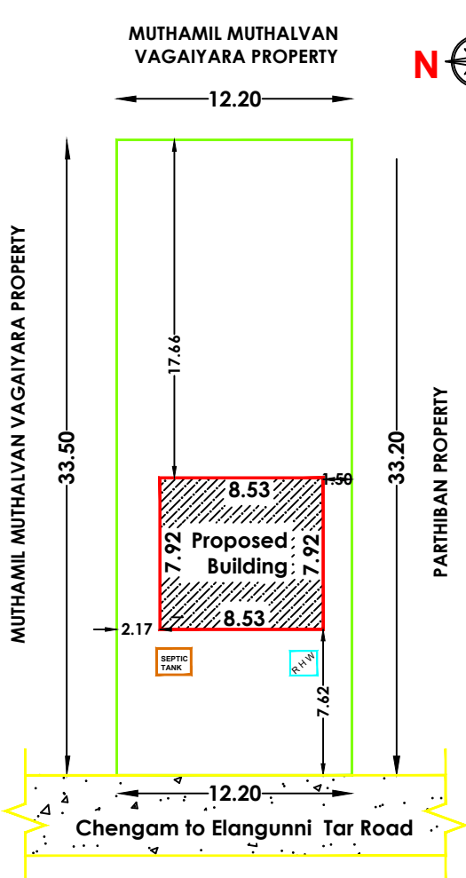
SITE PLAN
