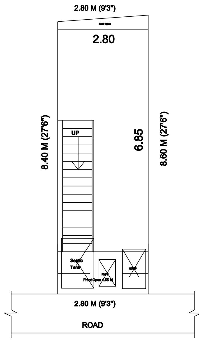
SITE PLAN
