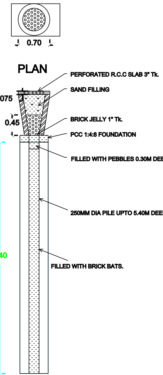
PERCOLATION PIT SECTION OF RAIN WATER
