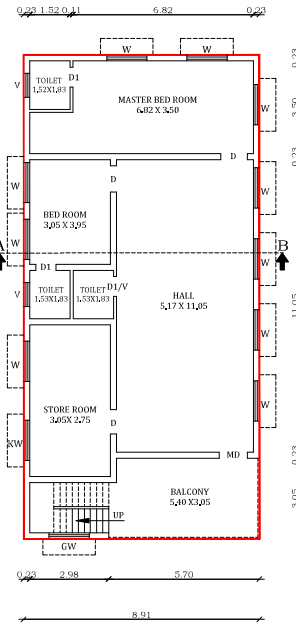
PROPOSED FIRST FLOOR PLAN
