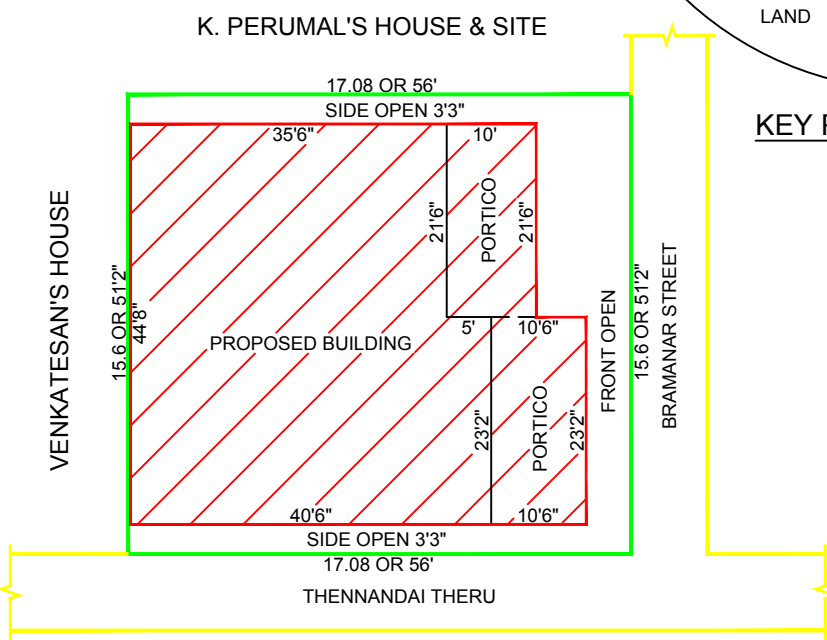
SITE PLAN SCALE: 1" = 33'
