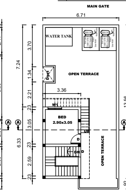
FIRST & TERRACE FLOOR PLAN
