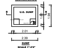
SUMP SCALE 1"=2'0"
