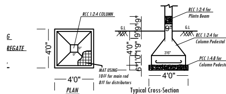
FOOTING DETAILS
