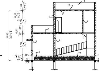
SECTION ON "JS"
