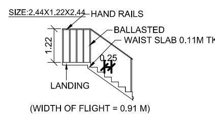
STAIRCASE DETAIL
