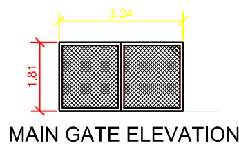
MAIN GATE ELEVATION
