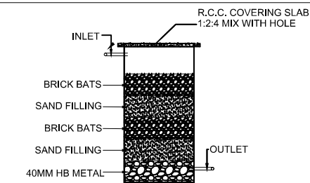
WASTE WATER RECYCLED UNIT
