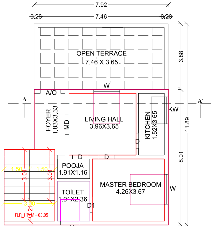
PROPOSED FIRST FLOOR BUILDING
