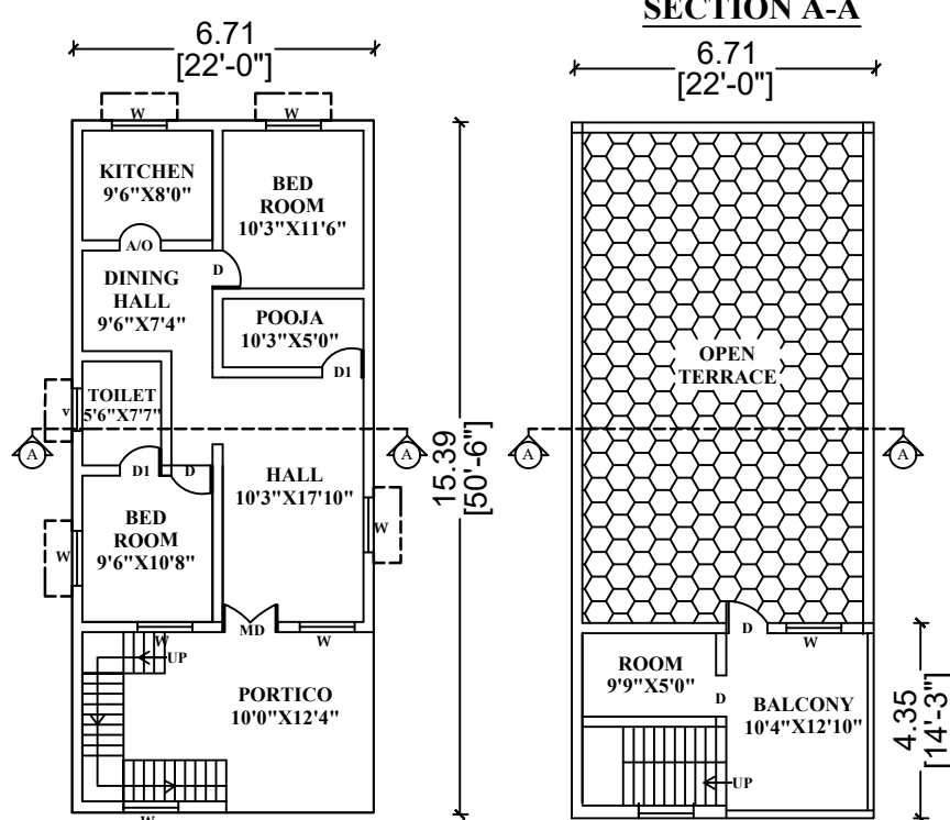
SOUTH FACING GROUND FLOOR PLAN BLOCK - 1
