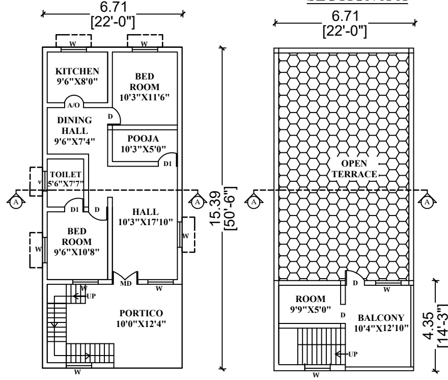
SOUTH FACING GROUND FLOOR PLAN BLOCK - 2
