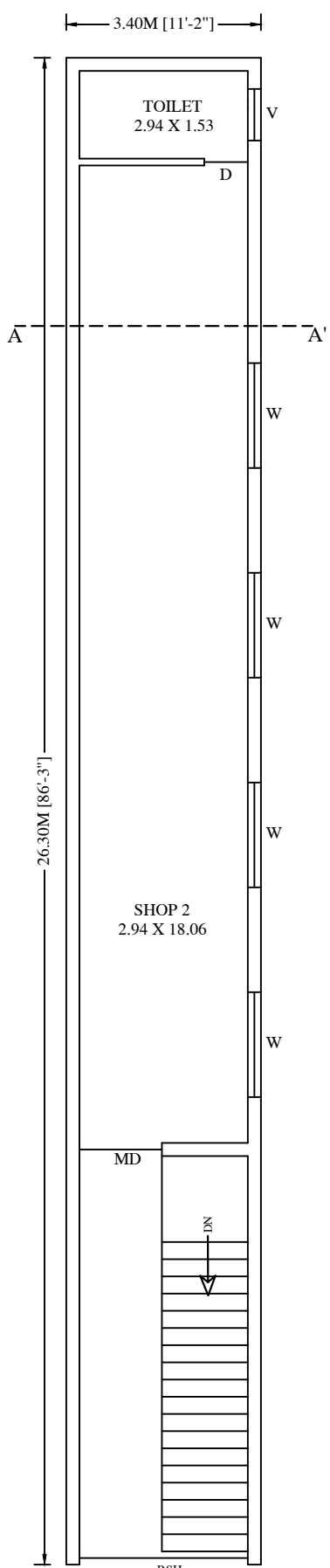
PRO.FIRST FLOOR PLAN
