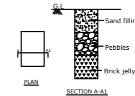
SIZE 1.50 X 1.00 RAIN WATER HARVESTING SYSTEM
