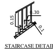
STAIRCASE DETAIL
