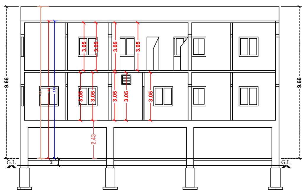
CROSS SECTION ON A-B
