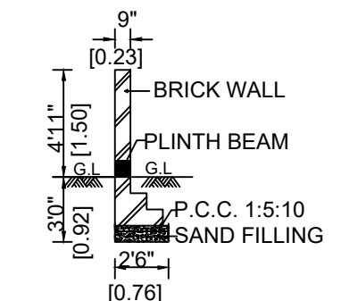
SECTION - CC
