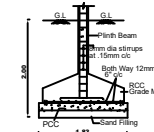
SECTION OF FOOTING
