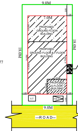
SITE PLAN
