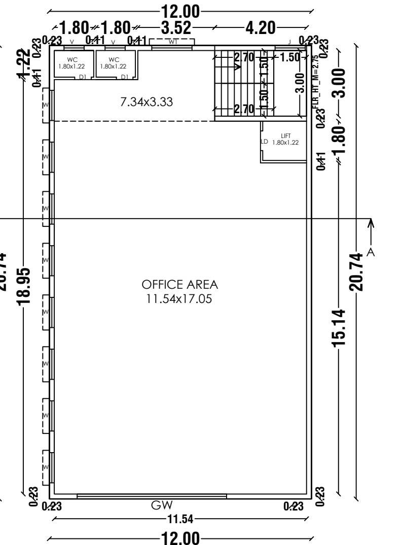
FIRST FLOOR
