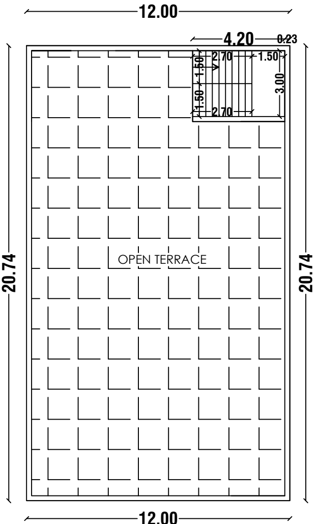
TERRACE FLOOR
