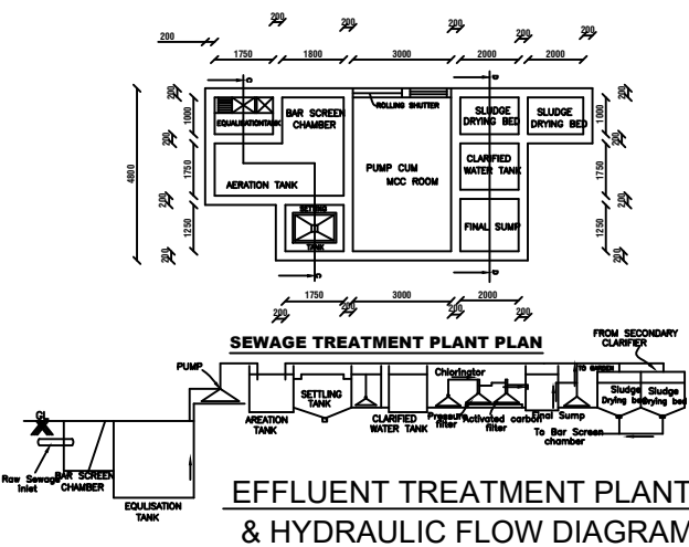
EFFLUENT TREATMENT PLANT & HYDRAULIC FLOW DIAGRAM
