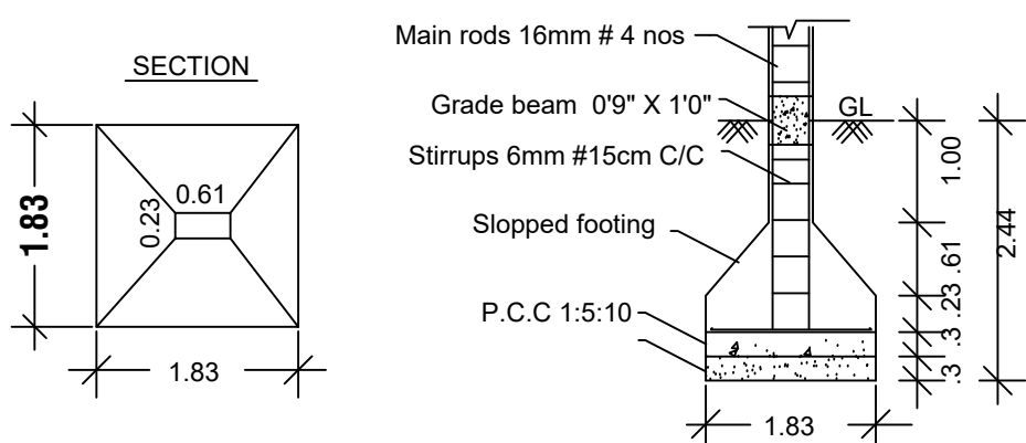
COLUMN DETAILS
