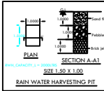
RAIN WATER HARVESTING PIT
