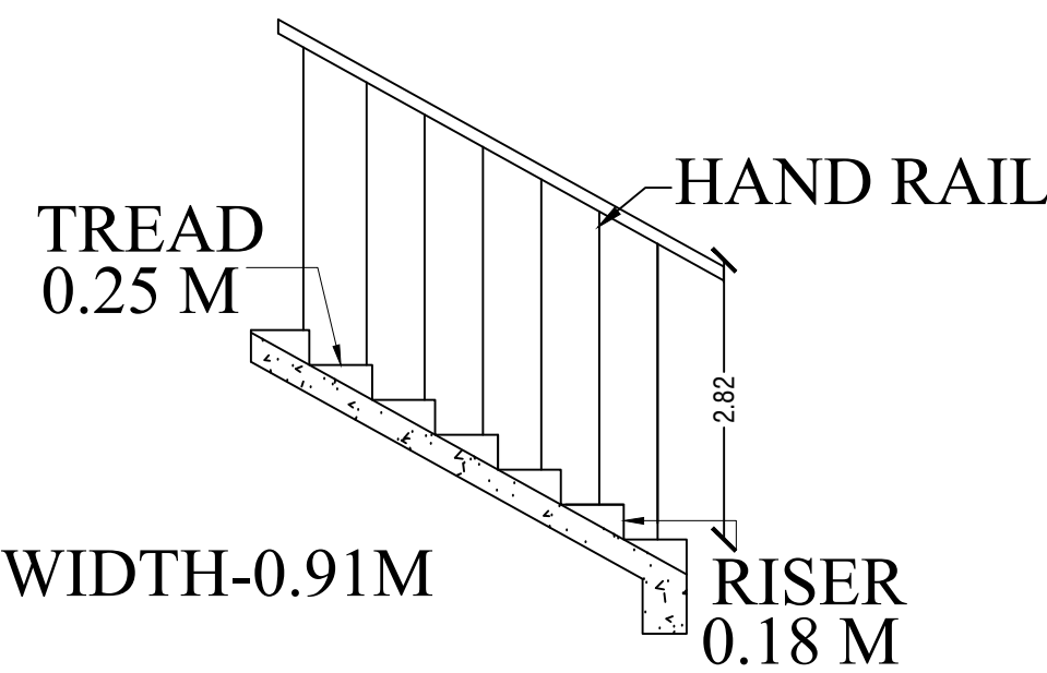
STAIRCASE DETAILS
