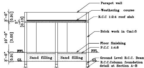
SECTION ON 'SA'
