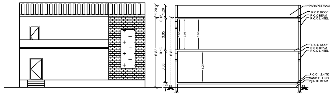
FRONT ELEVATION.
