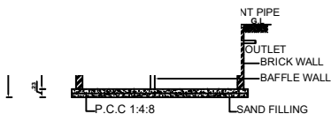
SECTION 'Y-Y'
