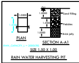
RAIN WATER HARVESTING PIT
