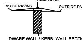
DWARF WALL / KERB WALL SECTION
