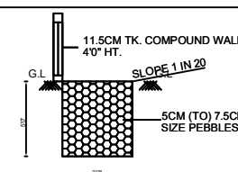
DETAIL OF PEBBLE BED ARRANGEMENT
