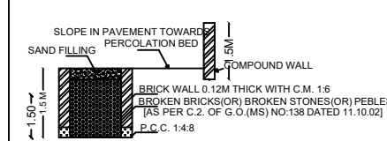
SECTION OF RAIN WATER PERCOLATION BED RWH CAPACITY L=5000LTRS
