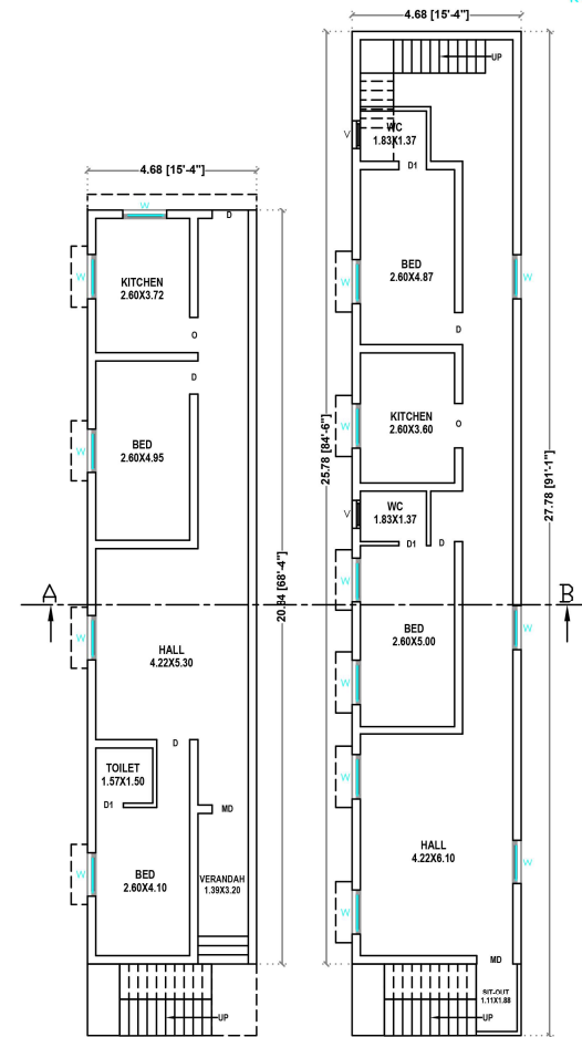
EXI.GROUND FLOOR
