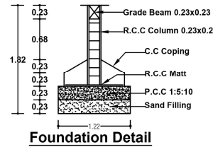
Foundation Detail
