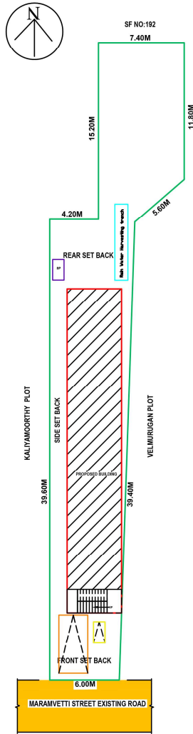
SITE PLAN
