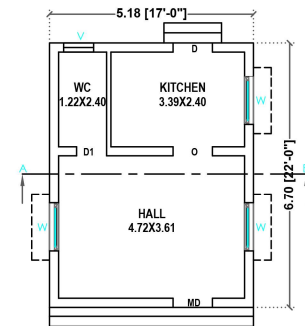
PRO.GROUND FLOOR
