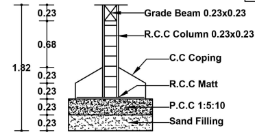
Foundation Detail
