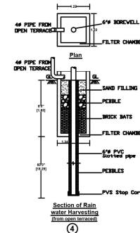
Section of Rain water Harvesting through Borewell
