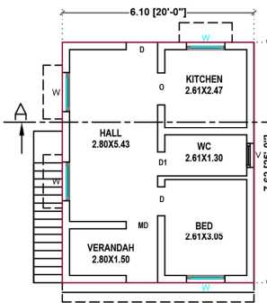
EXI.GROUND FLOOR
