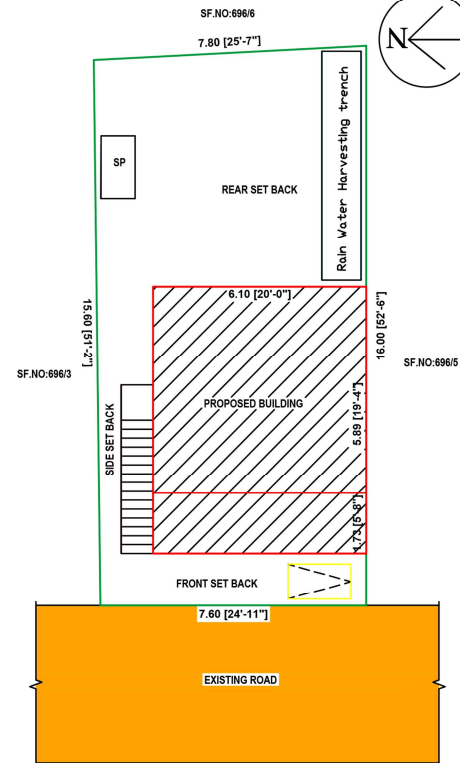
SITE PLAN
