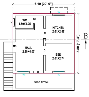
PRO.FIRST FLOOR
