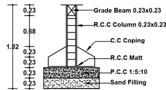
Foundation Detail
