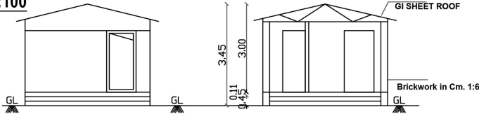
FRONT ELEVATION
