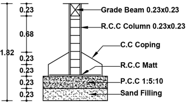
Foundation Detail
