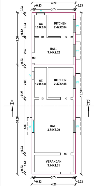
PRO.GROUND FLOOR BLOCK1&2
