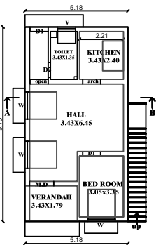
PRO., GROUND FLOOR PLAN
