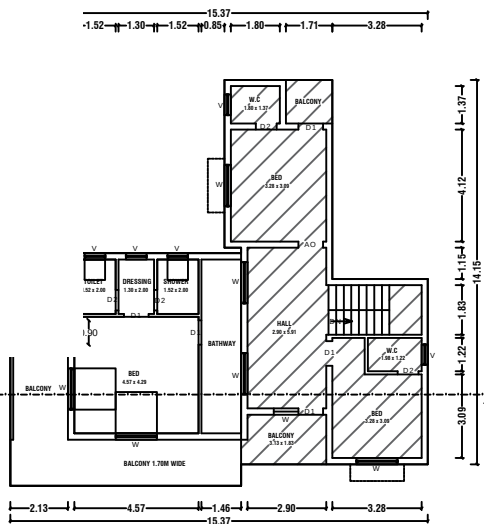
PROP.FIRST FLOOR PLAN
