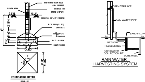
FOUNDATION DETAIL
