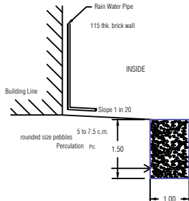
WASTE WATER RECYCLING SYSTEM:
