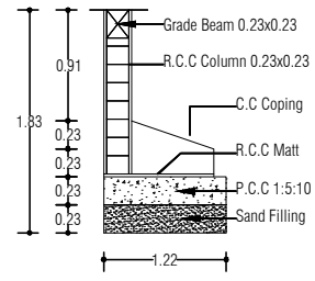
Foundation Details
