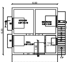
PRO. GROUND FLOOR PLAN
