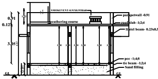
SECTION ON-AB
