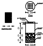
RAIN WATER FILTRATION SYSTEM
