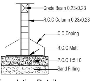
Foundation Detail
