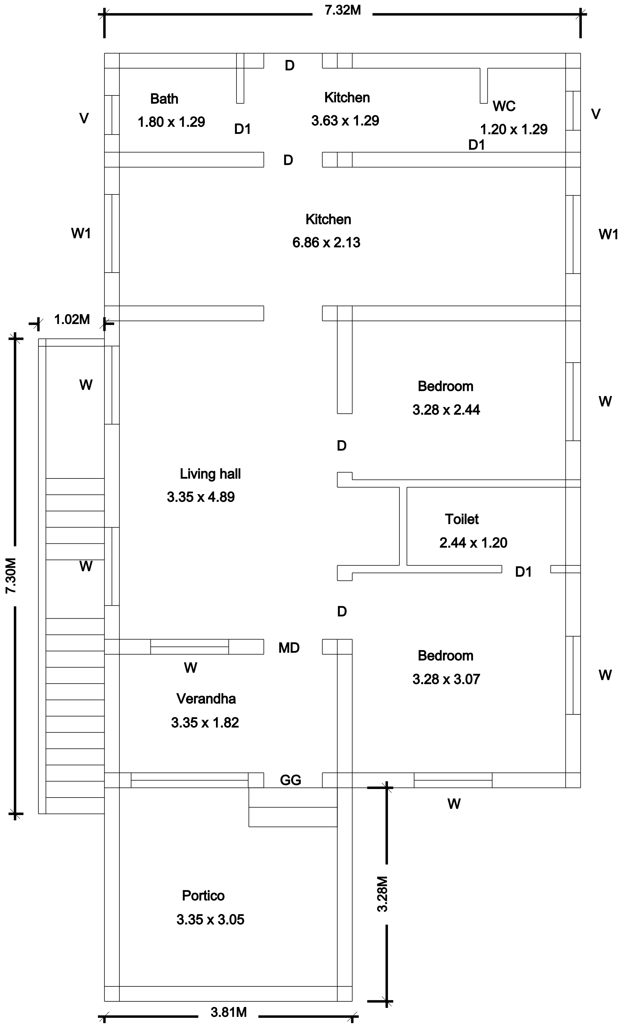
GROUND FLOOR
